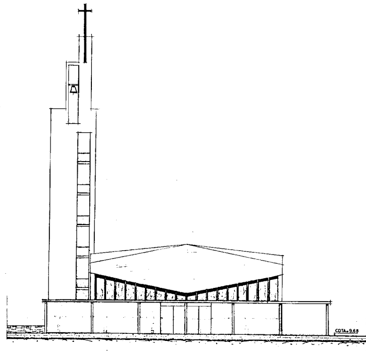
FACHADA PRINCIPAL
